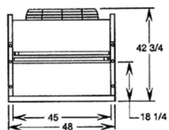
END VIEW: Single Fan-Width Models
