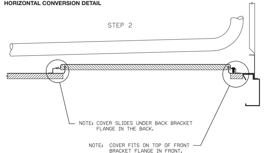
FIGURE 11 HORIZONTAL CONVERSION DETAIL
