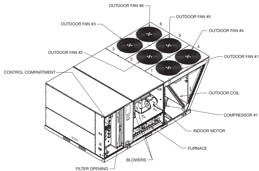
FIGURE 5 COMPONENT LOCATIONS
