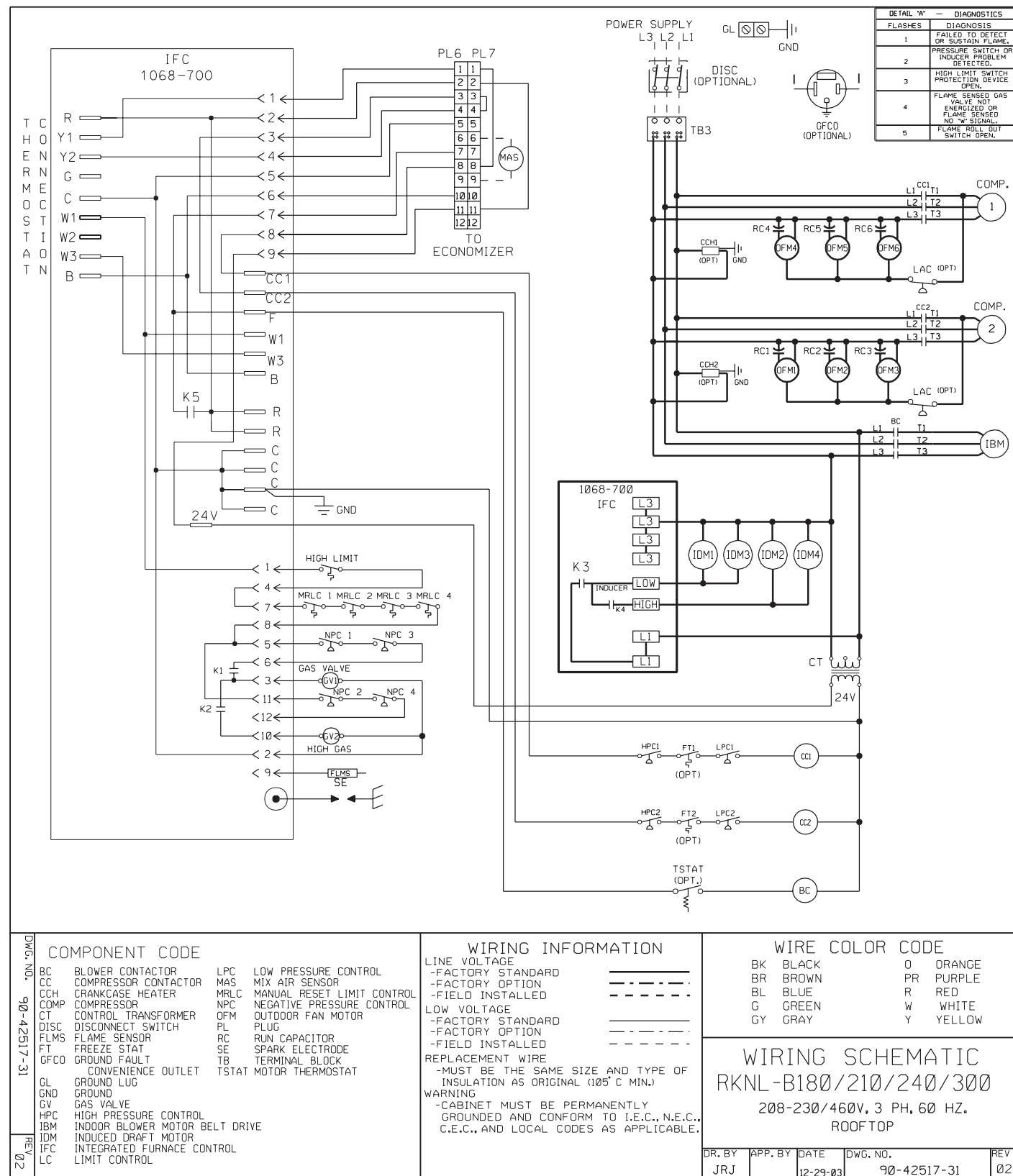
FIGURE 27 RKNL SERIES
