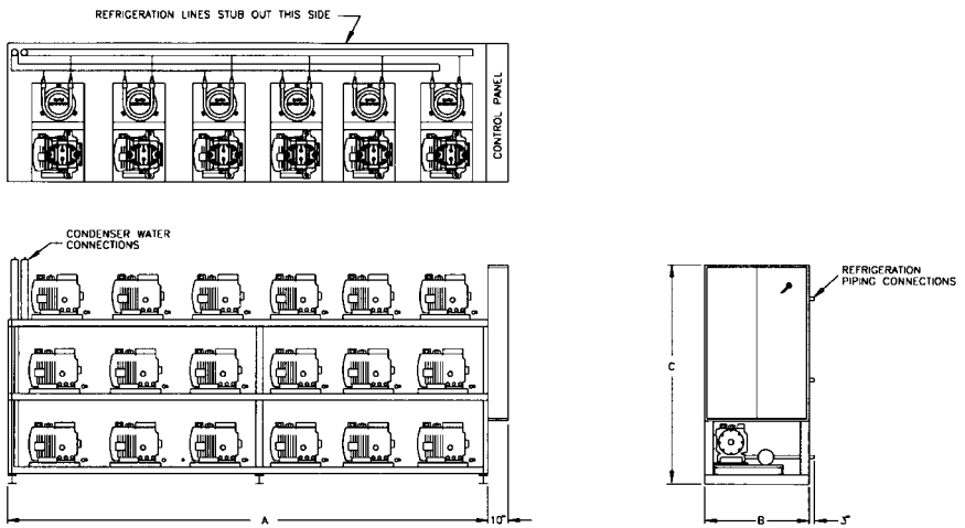
ENVIRO COOL COMPRESSOR RACKS
