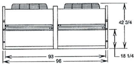
END VIEW: Double Fan-Width Models
