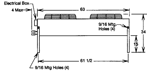
Two-Fan Units
