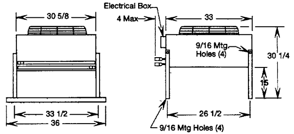
One-Fan Units
