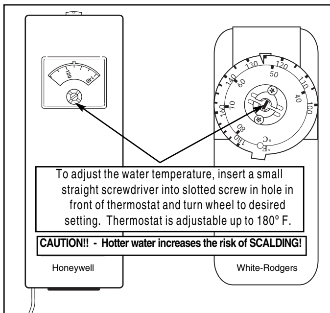
Figure 11. — Thermostat adjustment
