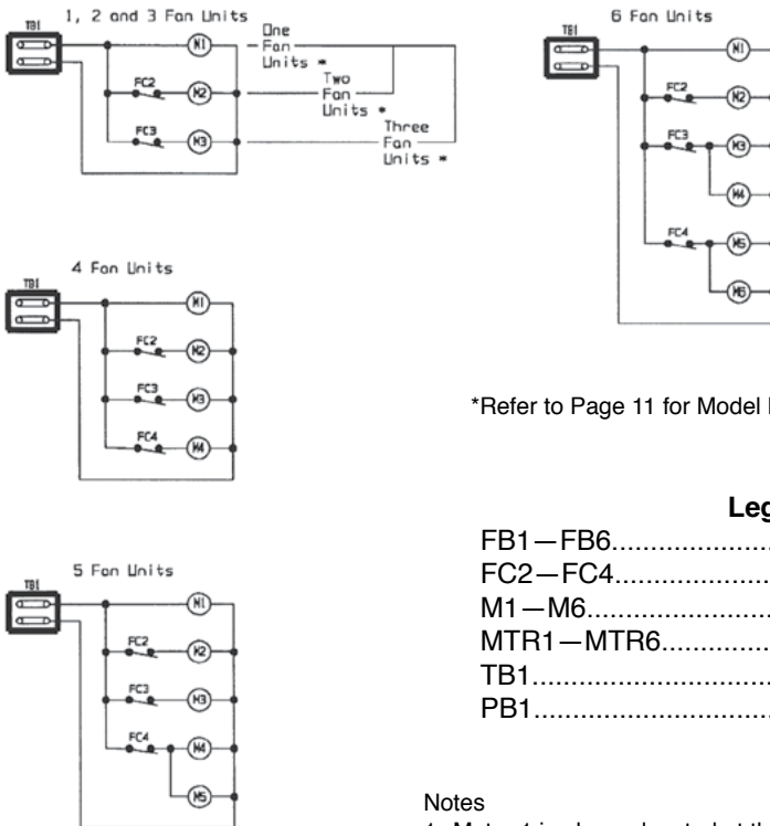
Control Wiring
