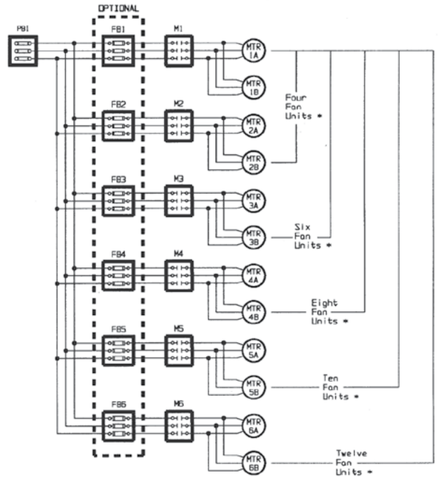
Figure 5: — Double Fan Width Units Power Wiring
