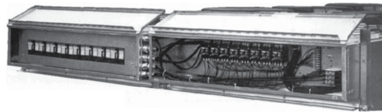
Individual Fan Contactor and Circuit Breaker option shown
