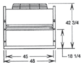
END VIEW: Single Fan-Width Models
