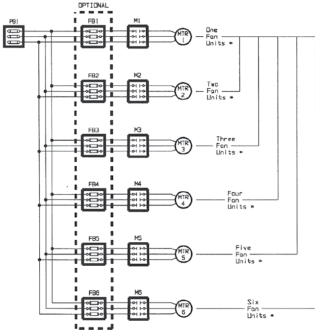
Figure 4: — Single Fan-Width Units Power Wiring
