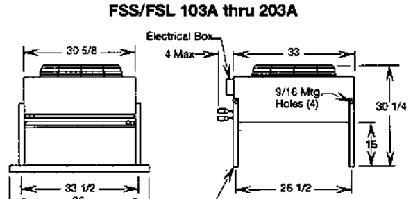
One-Fan Units
