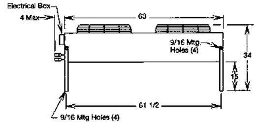
Two-Fan Units
