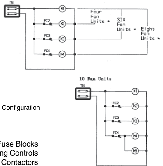
Control Wiring
